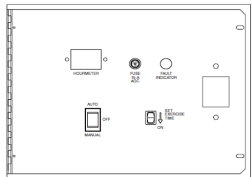
Generac Pre-R Liquid Cooled Control Panel
